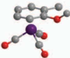
NMR enantiodifferentiation
