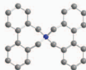
NMR enantiodifferentiation
