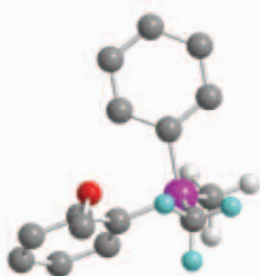
NMR enantiodifferentiation
